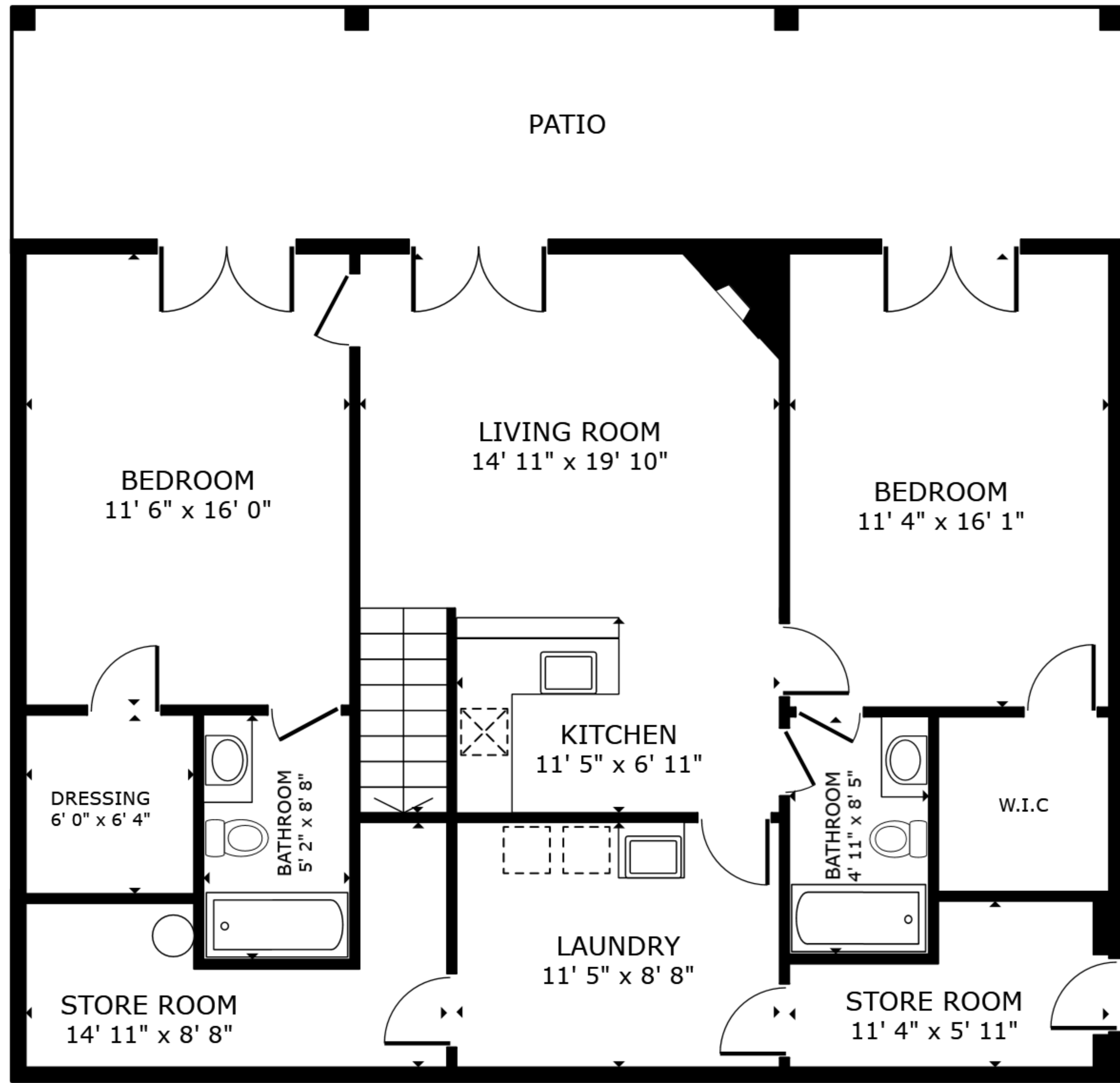
FLOOR 1
