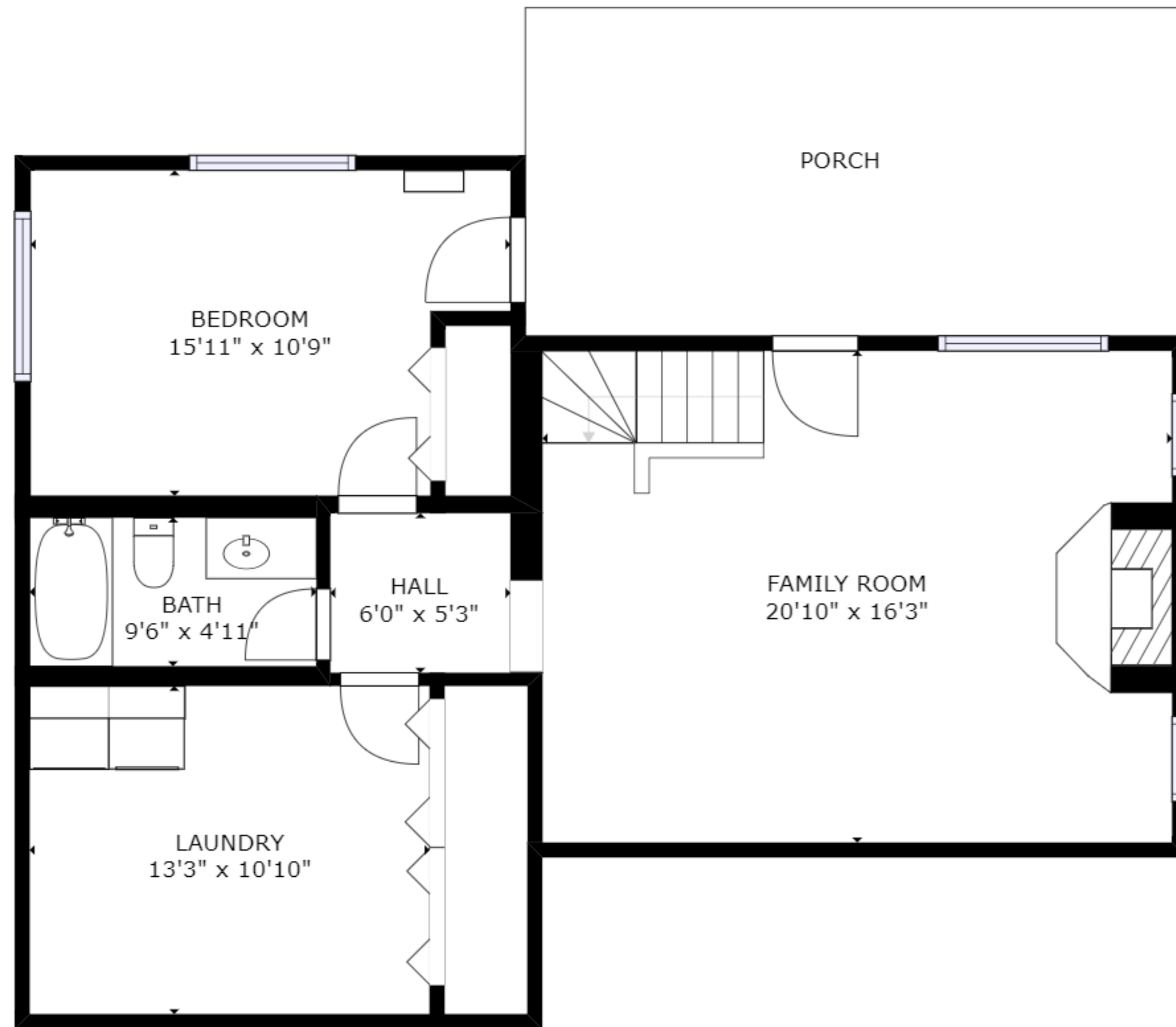
FLOOR 1
