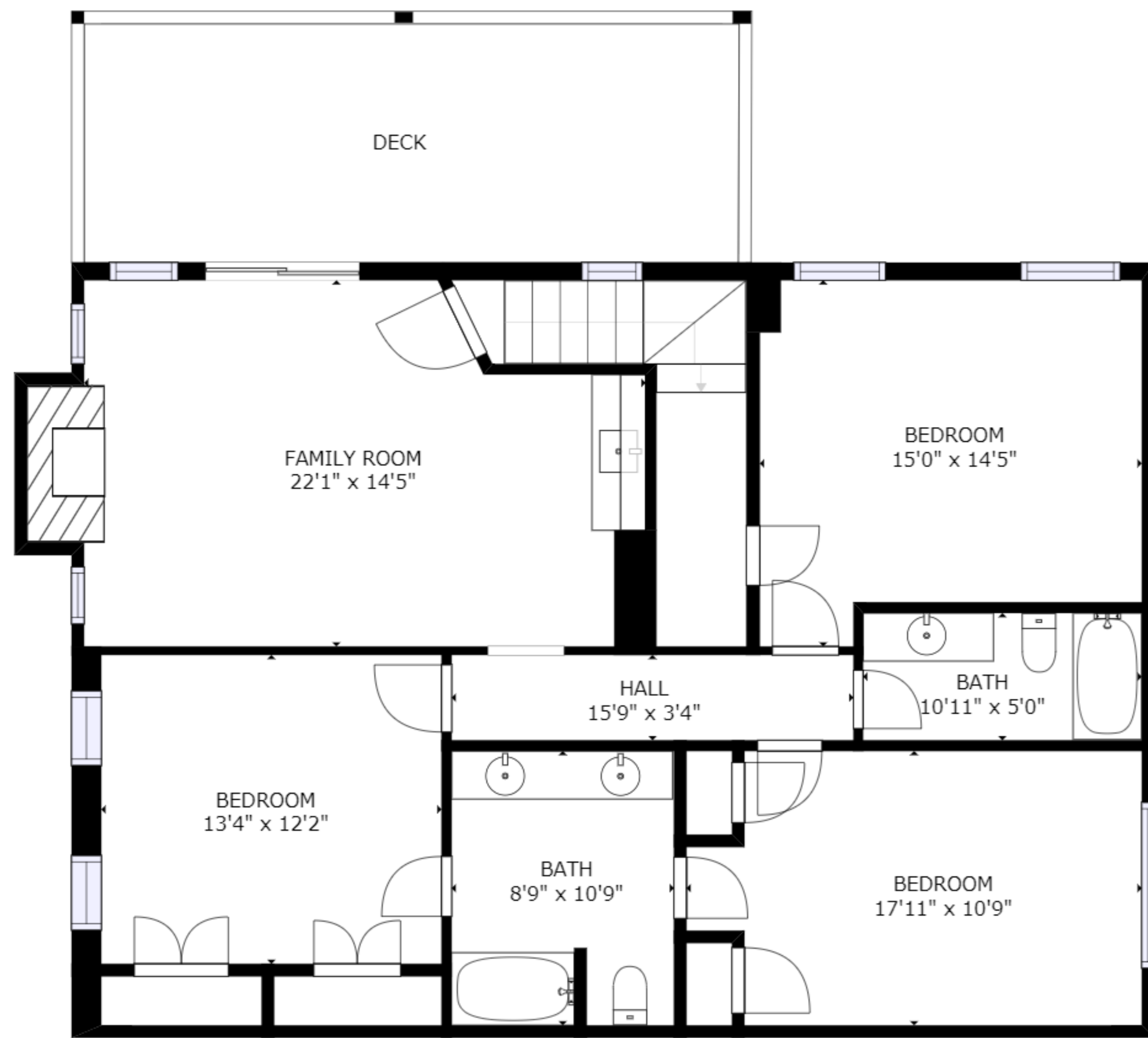
FLOOR 1
